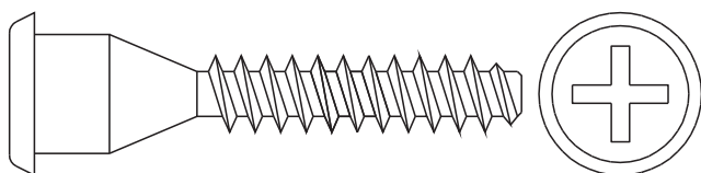
A10- Tornillo \varnothing 7,0 \times 40 (4x)
