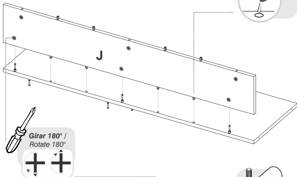
Tarugo/ Fluted Dowel Pin
