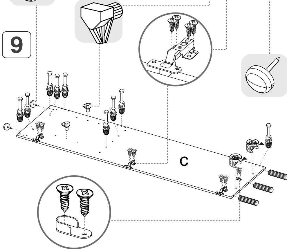
Soporte Tubo ovalado/ Closet Rod Support
