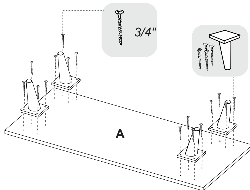
Tornillo Ensamble 3/4"/ Drywal Screw 3/4"
