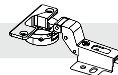
BISAGRA INTERIOR 35MM
